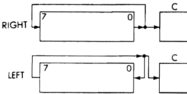
Fig. 4.12: Eight-Bit Rotation
