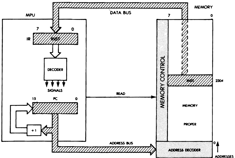
Fig. 2.7: Automatic Sequencing
